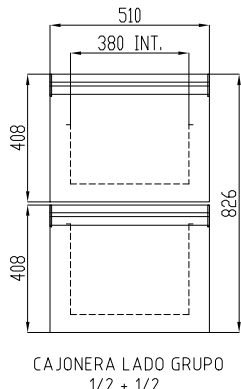
CAJONERA 1/2 + 1/2
