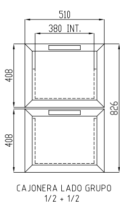
CAJONERA 1/2 + 1/2
