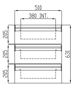
CAJONERA 1/3 + 1/3 + 1/3
