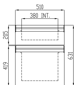
CAJONERA 1/3 + 2/3
