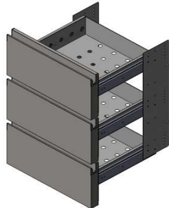
23. KIT CAJONES 1/3
